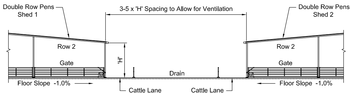
Figure 5. Typical end elevation – fully covered single row shed
